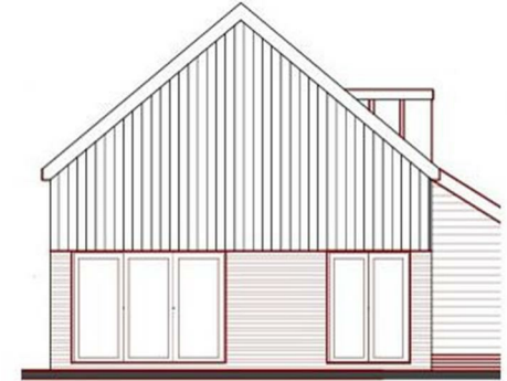
West Elevation
